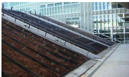
In the pitched roof area Georaster®-elements have been applied to hold the substrate.
