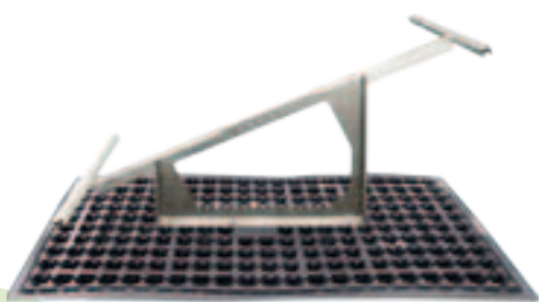
Solar Base Frame with Adapter Profiles to increase the mounting distance
