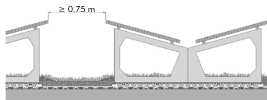
Solar Substructure Type "Butterfly"
