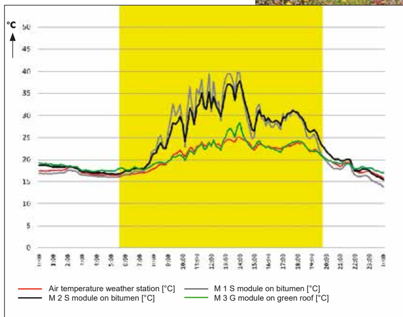
Graph: example of temperature graph recorded on a day in July. The temperature of the modules over a bituminous membrane (black and grey lines) rises to almost 40 °C, while that of the module on the green roof (green line) does not go beyond a maximum of 27 °C and is, therefore, close to the ambient temperature (red line).
