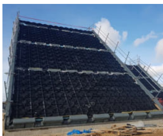
The 40–45° pitched steep roof areas are very well prepared with the system build-up Steep Pitched Green Roof with Georaster® elements.
